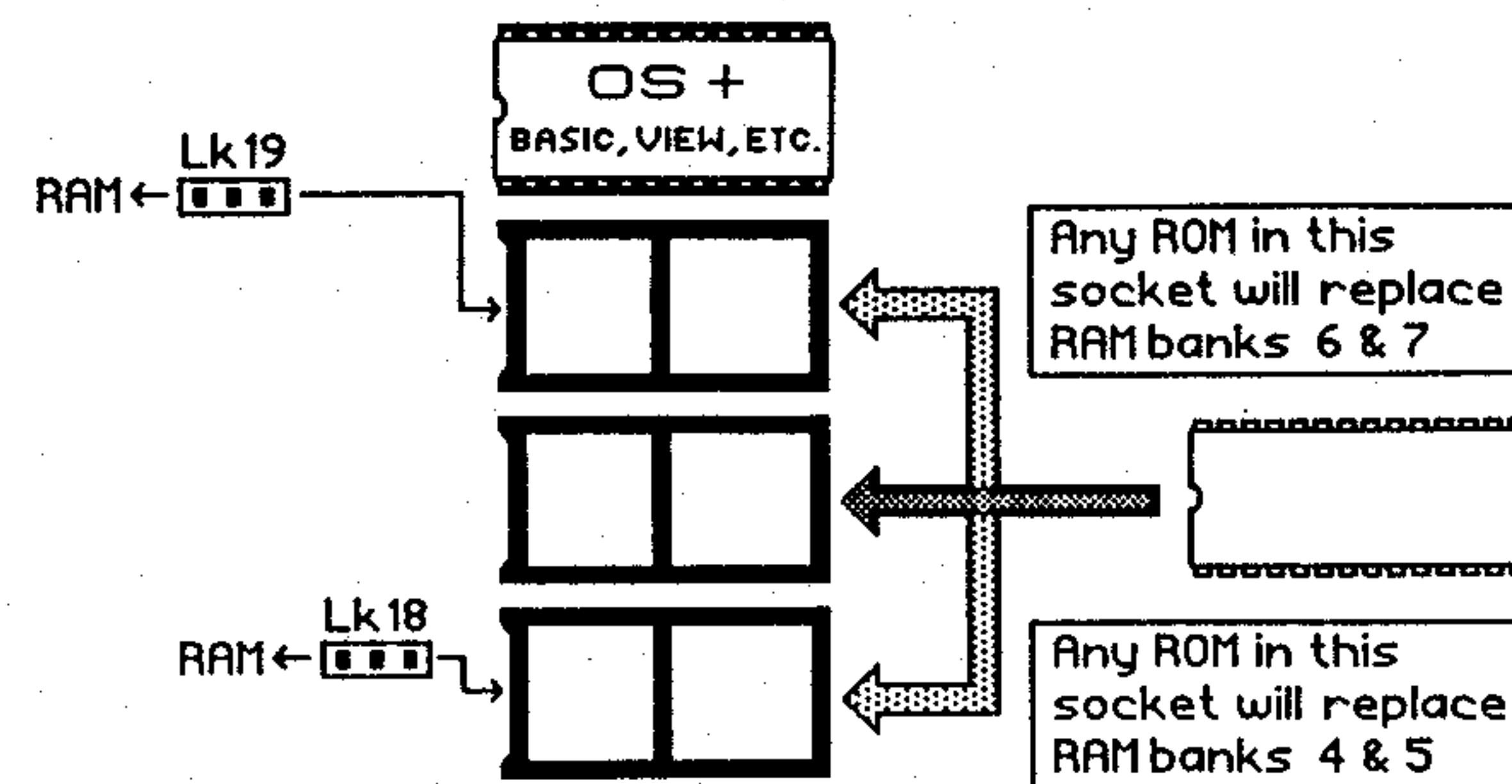
The ROM Sockets on the Master Series
