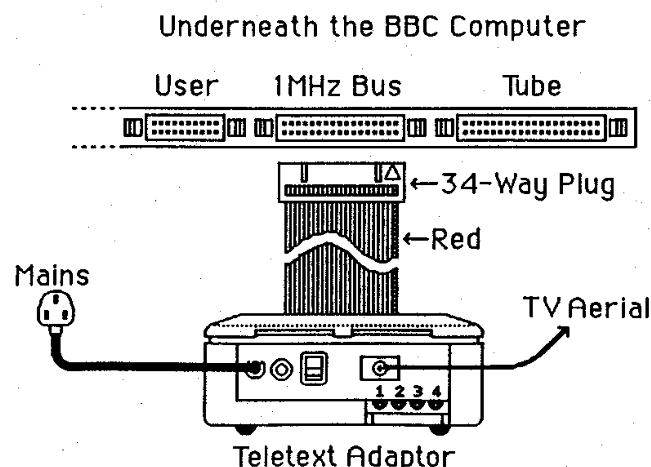
Figure 1 Connecting the Teletext Adaptor
