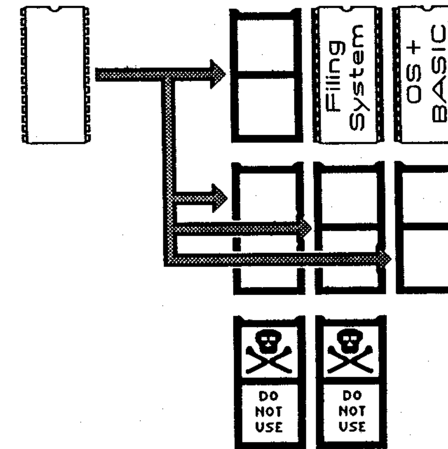
The ROM Sockets on the Model B+
